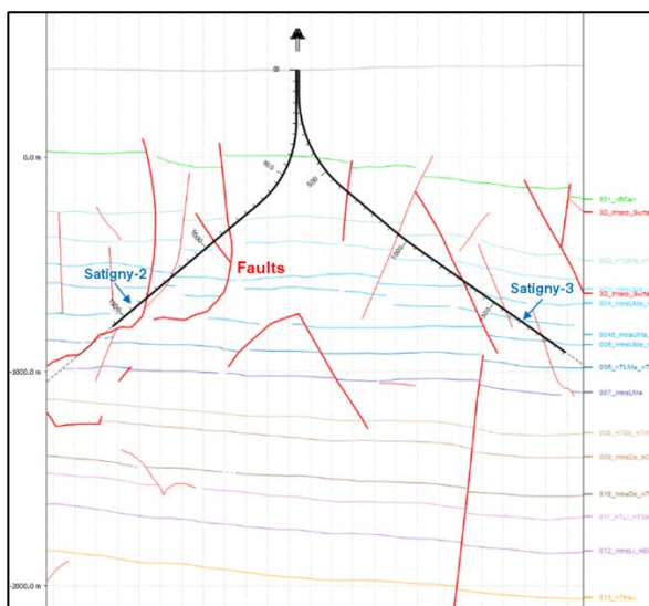
Figure 5: Cross section showing the planned trajectories for Satigny-2 and Satigny-3
