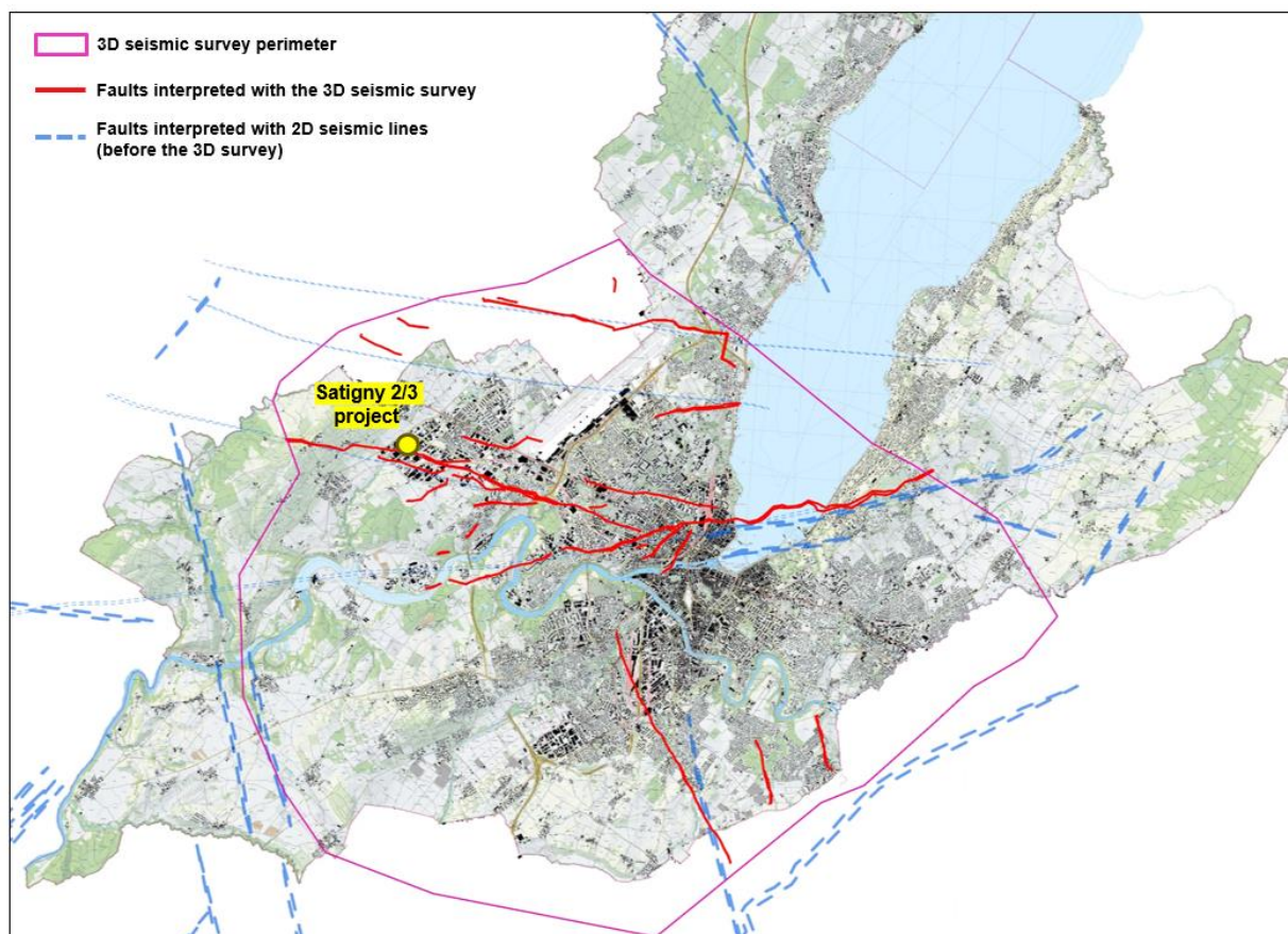
Figure 2: Localisation of the Satigny 2&3 project and major geological faults
