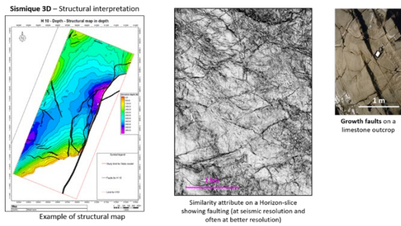
Figure 7 - Structural information obtained in a 3D seismic (mapping and similarity attribute), compared with a fractured limestone outcrop (on the right) [23 – DROUILLER et al., 2019]
