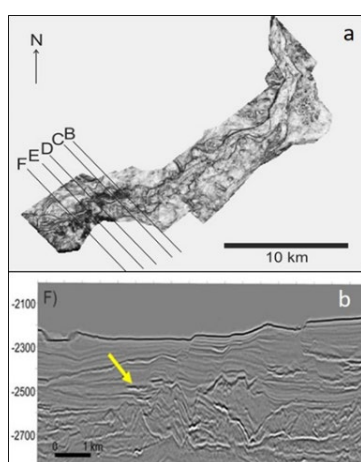
Figure 10– Horizon-slice (a) showing the fluvial system visible on the section (b) – [19 - ORTIZ-KARPF A. (2016)]
