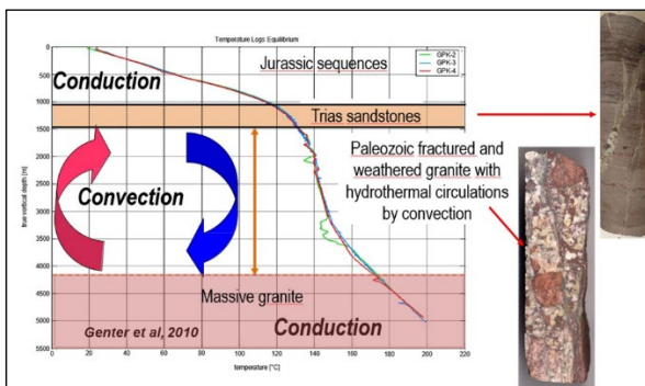
Figure 1 - Thermal profiles in boreholes at Soultz, in the upper Rhine graben [2 - GENTER & al., 2010]
