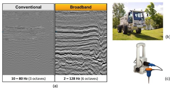
Figure 6 - ONSHORE 3D seismic acquisition - Progress realized with the 6 octaves (2-128 Hz) Broadband technique (a), courtesy of PDO, single vibrator (b) and single wireless geophone for use on URBAN SITES (c), courtesy of Sercel [23 – DROUILLER et al., 2019]
