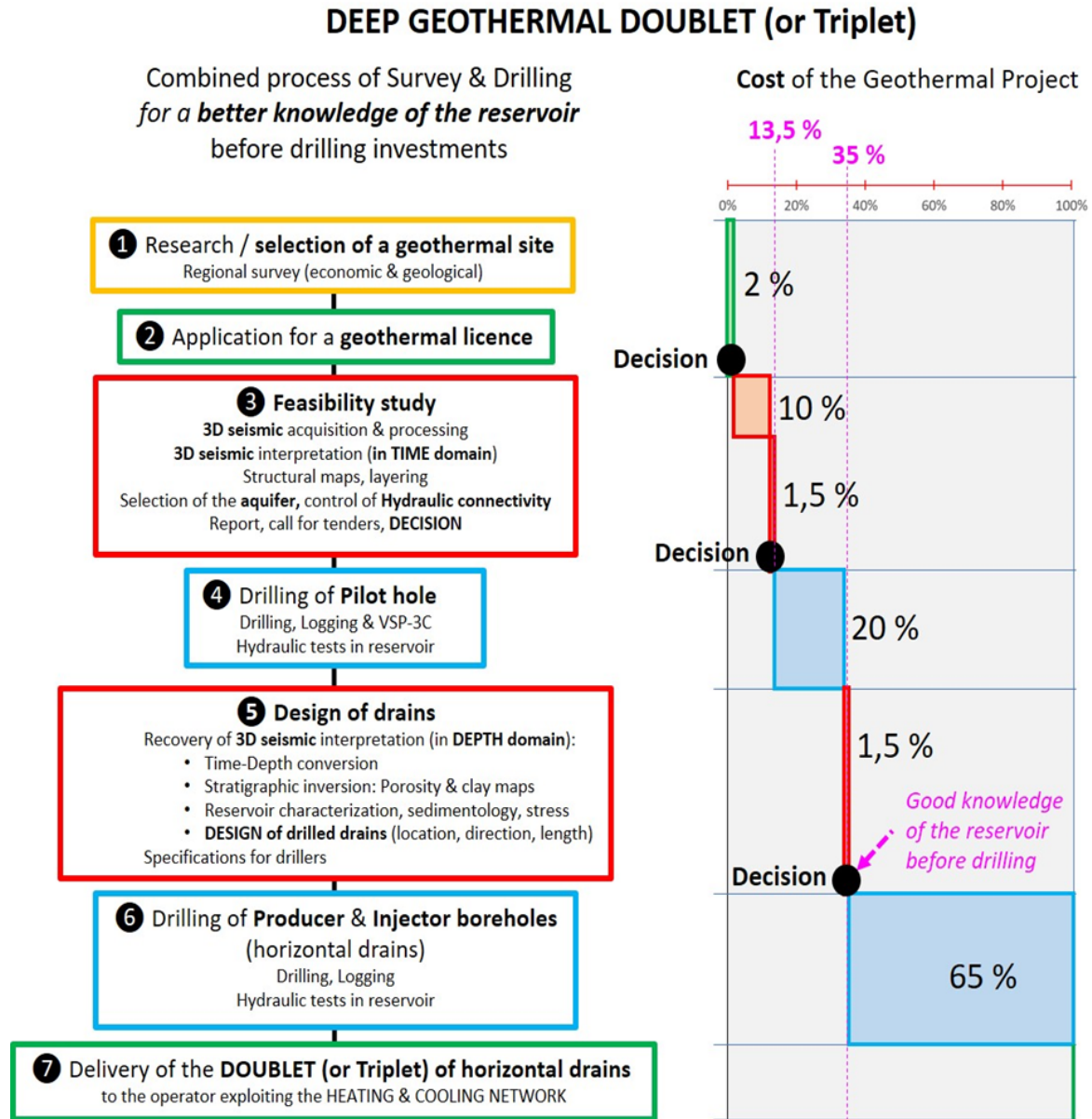
Figure 11 - Combined Process for the survey of the objective aquifer (stratified or fractured) and design of geothermal doublets/triplets before drilling investments [23 – DROUILLER et al., 2019]
