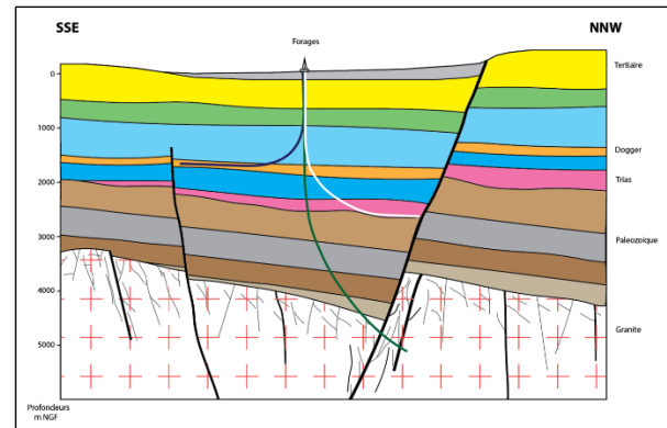
Figure 13 – Project for geothermal exploitation by several superimposed aquifers: two stratified reservoirs and a fractured aquifer along a regional fault affecting the granitic basement, using the same 3D seismic dataset [DROUILLER et al., 2019]
