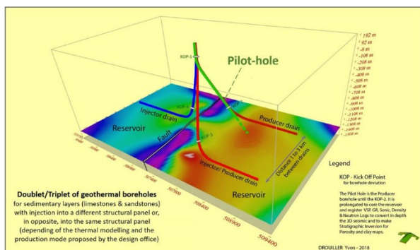
Figure 12 - Example of a geothermal triplet with horizontal drains inside the reservoir. The porosity map (simulation here) characterizes the reservoir in each side of the fault. The better knowledge of the reservoir allows to inject cold water in a different structural panel. The third drain allows to inject or produce hot water, giving the operator both options depending on the season and the needs of the heating and cooling network [23 – DROUILLER et al., 2019]
