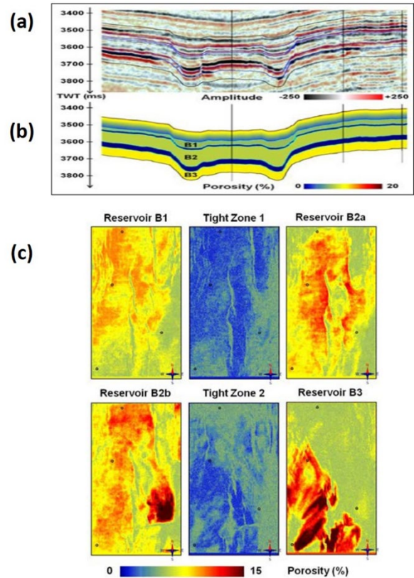
Figure 8 - Carbonate Reservoir (Brazil Offshore) – Seismic section (a), initial porosity model (b) and maps (c) showing lateral evolution of the porosity in the different reservoirs and intermediate impermeable layers obtained by petrophysical inversion of the 3D seismic dataset [17 – COLEOU Th. & al. – 2012]
