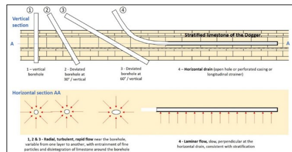
Figure 2 - Type of flow in the aquifer depending on the geometry of the borehole [23 – DROUILLER et al., 2019]
