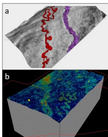
Figure 9 – Examples of fluvial systems which can be observed in 3D seismic (Courtesy of Eliis) [23 – DROUILLER et al., 2019]
