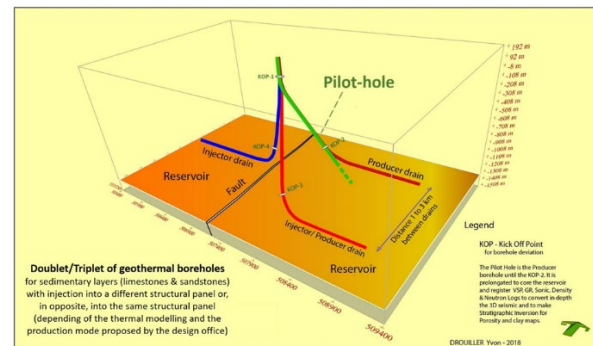
Figure 4 - Example of architecture of boreholes with horizontal drains inside the reservoir which needs a better knowledge of the reservoir to manage (or not) the hydraulic connection. Where the design office will inject cold water? In a different structural panel or, in opposite, in the same structural panel? Faults location is needed [23 – DROUILLER et al., 2019]
