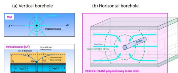
Figure 3 - Comparison of flows in a vertical borehole (a) and in a horizontal drain (b) - [23 – DROUILLER et al., 2019]
