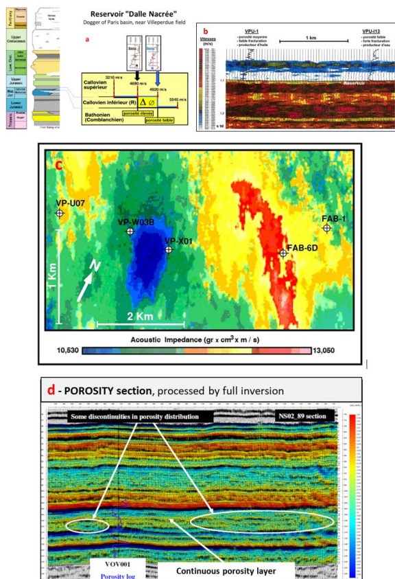
Figure 5 - Reservoir “Dalle Nacrée”: Variations of velocity and acoustic impedance explain POROSITY variations on Sonic log (a), 2D seismic profile (b) and 3D vibro-seismic horizon slice (c) – Variations of POROSITY on an inverted seismic section (d) - PICOREF project made in 1991-1993 by DHYCA to promote oil exploration in the Paris Basin [5- MOUGENOT D. et LAYOTTE P.C. - 1996]
